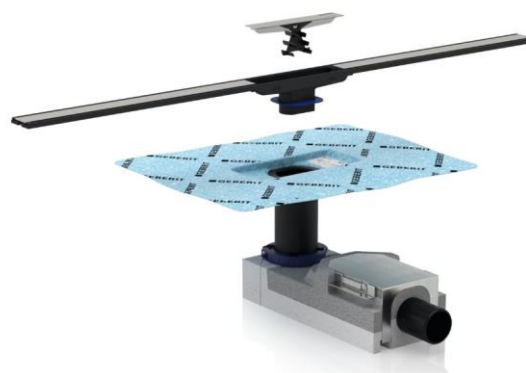
Fig. 2 Geberit gulvsluk for renne - Cleanline Figur: Geberit AS
